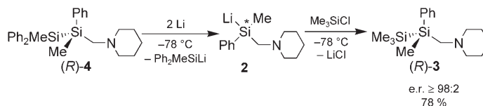
Scheme 2. Synthesis of ( R )- 3 by cleavage of the Si–Si bond in ( R )- 4 with lithium.
