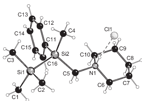
Figure 1. Molecular structure and numbering scheme of (R)-3·HCl in the crystal (Schakal plot; molecule 1 of two molecules). Selected bond lengths [Å]: Si1–Si2 2.346(4), Si2–C4 1.884(7), Si2–C5 1.896(7).
