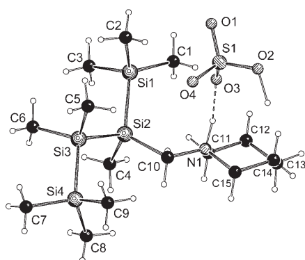
Figure 2. Molecular structure and numbering scheme of (R)-7·H 2 SO 4 in the crystal (Schakal plot; molecule 1 of two molecules). Selected bond lengths [Å] and angles [°]: Si1–Si2 2.3683(19), Si2–C4 1.890(5), Si2–C10 1.915(5), Si2–Si3 2.3508(18), Si3–Si4 2.350(2); C4–Si2–C10 107.6(2), C4–Si2–Si3 107.80(17), C10–Si2–Si3 103.88(15), Si3–Si2–Si1 110.80(7), Si4–Si3–Si2 111.94(7), N1–C10–Si2 119.6(3), Si1–Si2–Si3–Si4 –176.62(7).
