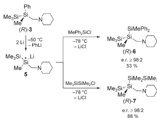
Scheme 3. Selective cleavage of the silicon–phenyl bond in the phenylsilane (R)-3 with lithium and synthesis of the trisilane (R)-6 and tetrasilane (R)-7.
